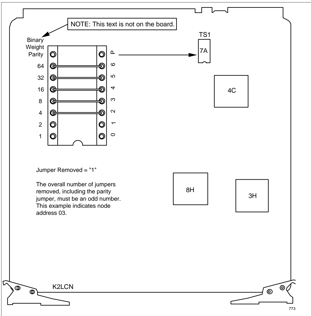
Figure 10-6 K4LCN Board (51402755-100) LCN Node Address Selection
